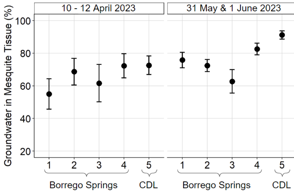
Figure 3. Groundwater fraction in plant tissues calculated from \delta^{18}\text{O} of the soil water, tree tissue water, and well water for each of the five sentinel sites in Borrego Springs and the reference site at Clark Dry Lake using a two-end mixing model as in equation 1. Well water is a value derived from the most-adjacent well sample possible.
